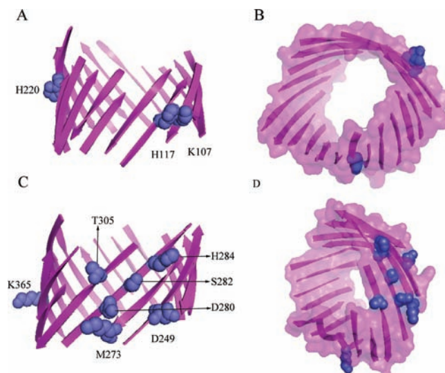
Figure 3. Predicted structures of the TM domains of Tom40 and Toc75. (a) Side view and (b) top view of the predicted structure of Tom40, along with the spatial location of unstable residues K107, H117, and H220. The triple mutant (K107L, H117L, and H220L) is predicted to be much more stable than the wild type monomeric protein; (c) Side view and (d) top view of the predicted structure of Toc75, along with the spatial location of the unstable residues D249, M273, D280, S282, H284, T305, and K365. Mutation D280L is predicted to have the most stabilizing effect on the monomeric form of Toc75 protein. The unstable residues in these proteins are likely to participate in protein–protein interactions.
